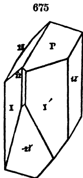
Hebronite, Maine.
